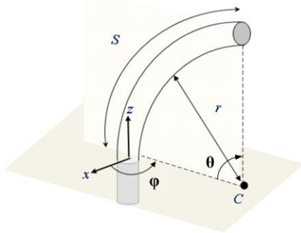
Figure 5. The pose of the tip of a continuum manipulator can be calculated by the arc parameters in the configuration space [17].
